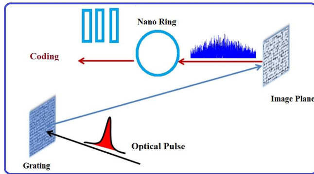
Fig. 1. Schematic diagram of the femtosecond pulse imaging gadget based totally on nonlinear micro ring resonators.
