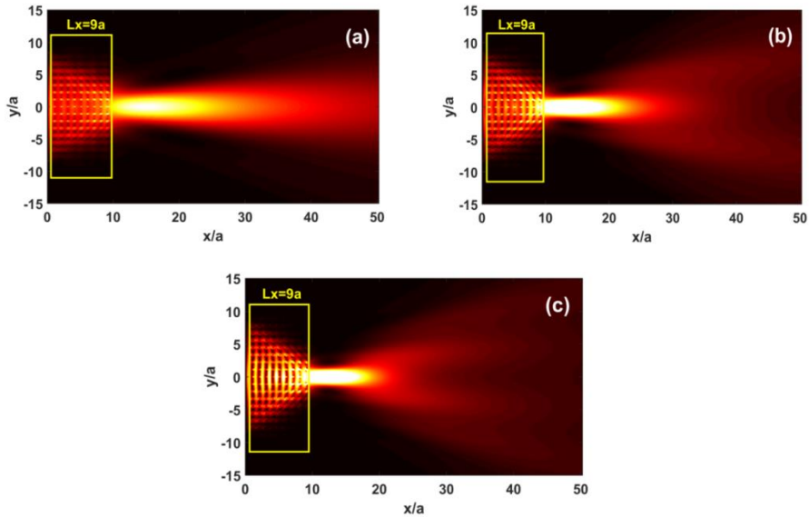
Fig. 6. The electromagnetic field propagation through GRIN PC structures with different refractive index of background material equal (a) n=1.4 , (b) n=1.8 and (c) n=2.1
