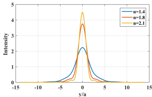
Fig. 7. The normalized intensity at focal point position of GRIN PC structures with different refractive index of background material
