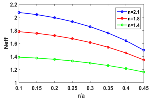
Fig. 4. The effective refractive index as a function of air hole radius for different value of refractive index of the background material
