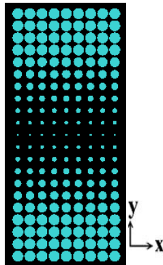
Fig. 1. The schematic representation of GRIN PC structure with parabolic refractive index
