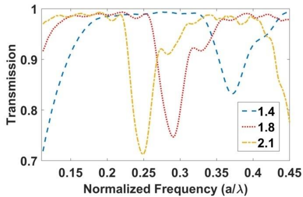
Fig. 5. The transmission spectrum of parabolic GRIN PC structures with different refractive index of background material calculated by the FDTD method
