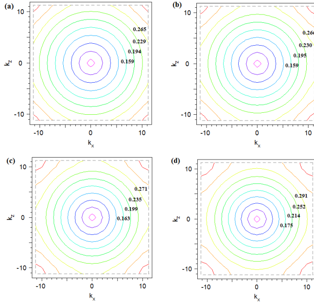
Fig. 2. Iso-frequency curves for PCs made of air holes in dielectric background in which the hole radius equal (a) 0.15a , (b) 0.25a , (c) 0.35a and (d) 0.45a
