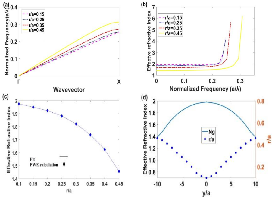
Fig 3. (a) Dispersion diagram along \Gamma -X direction for the first band, (b) The effective refractive index as a function of normalized frequency ( a/\lambda ), (c) The effective refractive index as a function of air hole radius at fixed frequency 0.18. (d) Effective refractive index and r/a for GRIN PC structure
