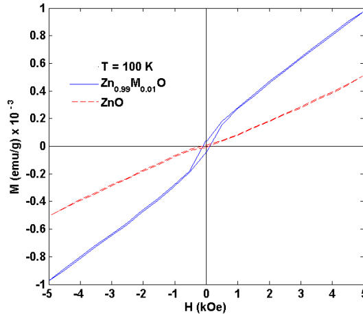
Fig. 1. Magnetization loops of \text{ZnO} and \text{Zn}_{0.99}\text{Mn}_{0.01}\text{O} at temperature 100 K
