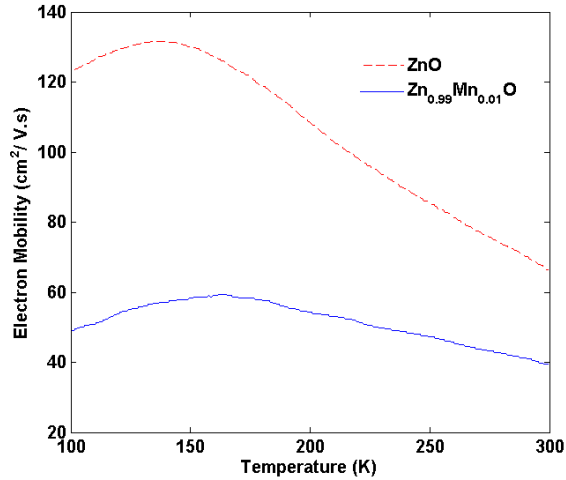
Fig.2. electron mobility for pure ZnO and Zn 0.99 Mn 0.01 O
