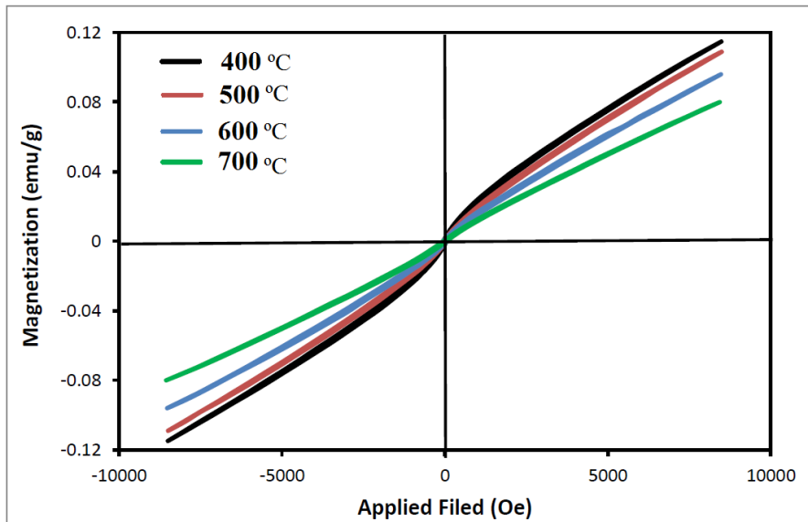
Fig. 4 Hysteresis loop at room temperature for nickel oxide nanoparticles with different cooking temperatures
