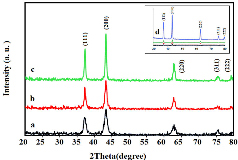
Fig. 1. XRD patterns of nickel oxide particle at different temperatures.
