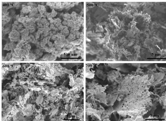
Fig. 2. FESEM images of nickel oxide at different calcination temperatures
