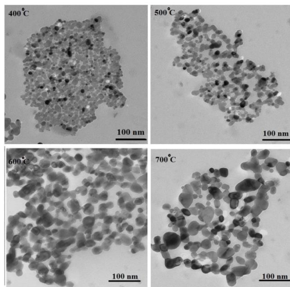
Fig. 3. TEM images of nanoparticles of nickel oxide at different temperatures.
