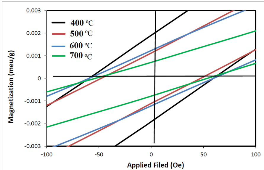
Fig. 5. The amount of residual magnetization and coercivity according to particles size
